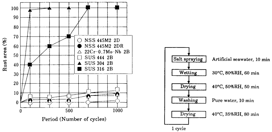
Fig. 3. Variation in Rust Area with Time After Weather Simulated Corrosion Test
